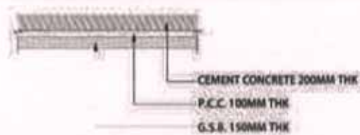
Figure 5 TYPICAL SECTION FOR CC ROAD CONSTRUCTION
