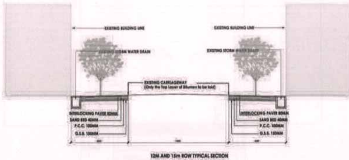
Figure 4 12M AND 15M ROW TYPICAL SECTION
