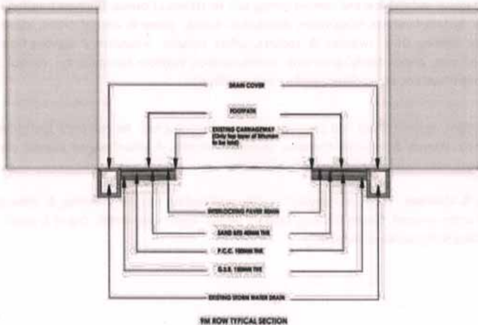
Figure 3 9M ROW TYPICAL SECTION
