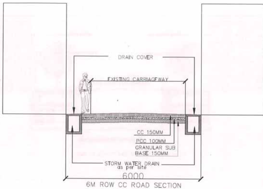
Figure 7 TYPICAL CROSS SECTION FOR CC ROAD CONSTRUCTION
